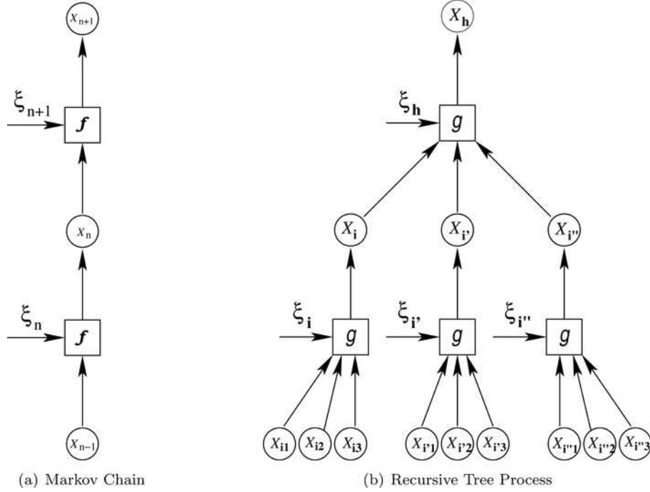
FIG. 1. On the left is a Markov chain represented as an iterated function system: X_n is the “output” of f with “inputs” \xi_n and X_{n-1} . On the right is an RTP; X_{\mathbf{i}} is the “output” of g with inputs \xi_{\mathbf{i}} and (X_{\mathbf{j}}, \mathbf{j} child of \mathbf{i}) . In the figure, \mathbf{h} is the parent of \mathbf{i} and \mathbf{i}', \mathbf{i}'' , ... are siblings of \mathbf{i} .
