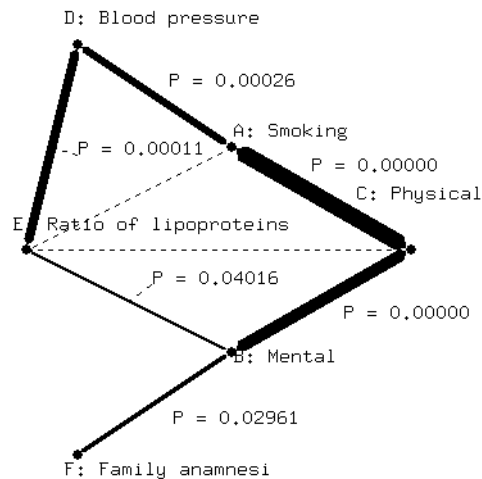
Figure 12.2: The result of a “Headlong Backward” on Graph-1 with added p -values. The bit-mat dump is created by Xlisp+CoCo.
