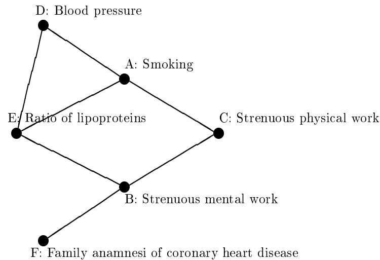
Figure 1.1: A final model from recursive coherent backward elimination with local and exact tests on data from Reinis et al. 81. The TeX-code of the figure is written by Xlisp+CoCo.
