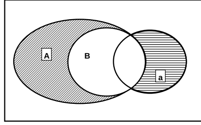
Figure 4.1: Collaps of M_A onto B containing a \cap A .
