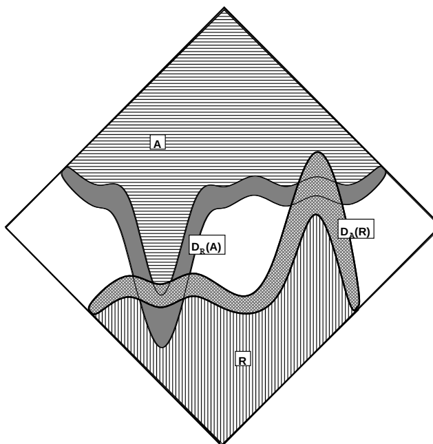
Figure 10.1: Weakly accepted and weakly rejected models and duals.
