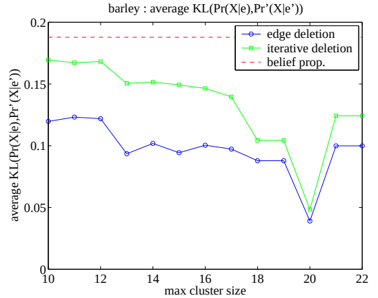
Figure 2: Quality of approximation in barley network
