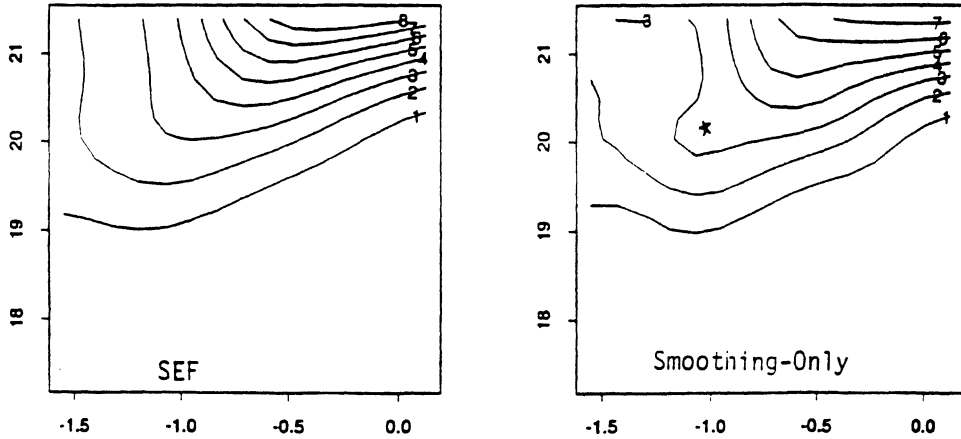
FIG. 4. Contour plots of the density estimates in Figure 3. The SEF contours (left panel) are much smoother than those from the smoothing-only estimate (right panel). The smoothing-only estimate has a weak second mode at the starred point.
