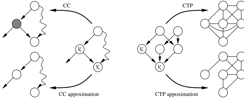
Figure 1: Reducing the complexity of cutset conditioning (CC) and clique-tree propagation (CTP) by removing arc V_r \rightarrow V_s .
