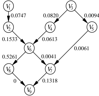
Figure 2: Information divergence for each arc in the digraph of an example belief network.
