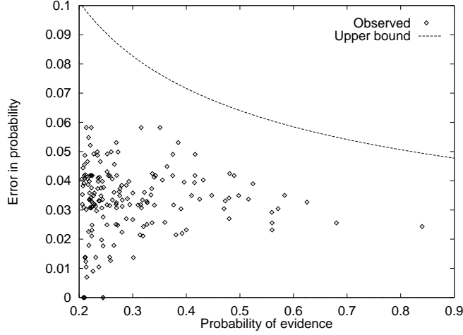
Figure 3: Posterior error in probabilities inferred from an approximated example belief network.
