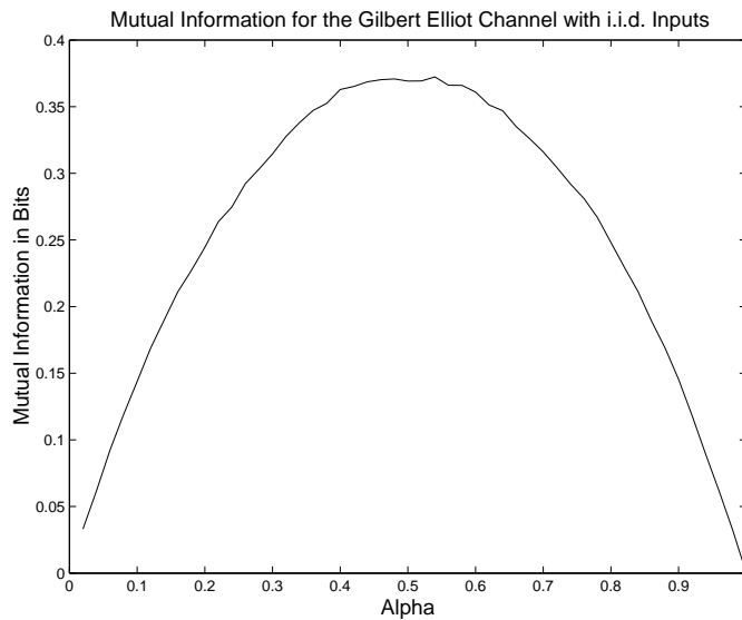
Fig. 2. Mutual Information of the Gilbert-Elliot Channel with i.i.d. Inputs.
