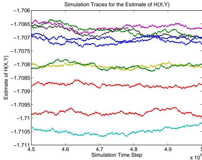
Fig. 1. Lyapunov exponent estimates from 10 sample paths of length 5.0 \times 10^5 . The estimate is \lambda_{XY} = -H(X, Y) for the ISI channel we consider in Section VII. Even though individual traces appear to converge we still receive different estimates from each trace.
