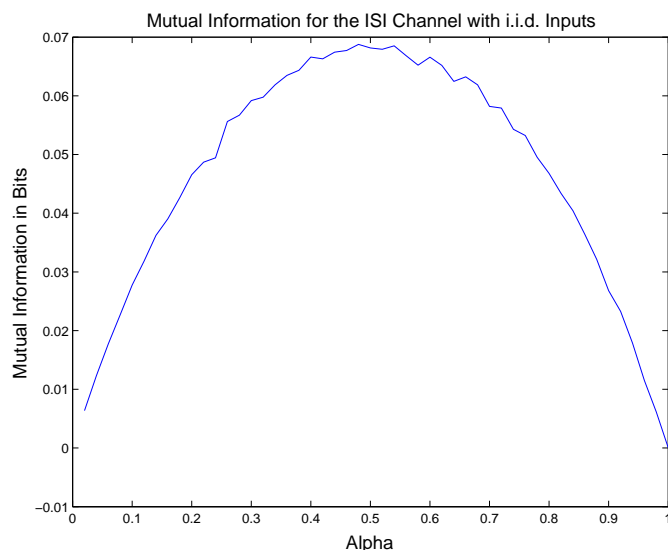
Fig. 4. Mutual Information of an ISI Channel with i.i.d. Inputs
