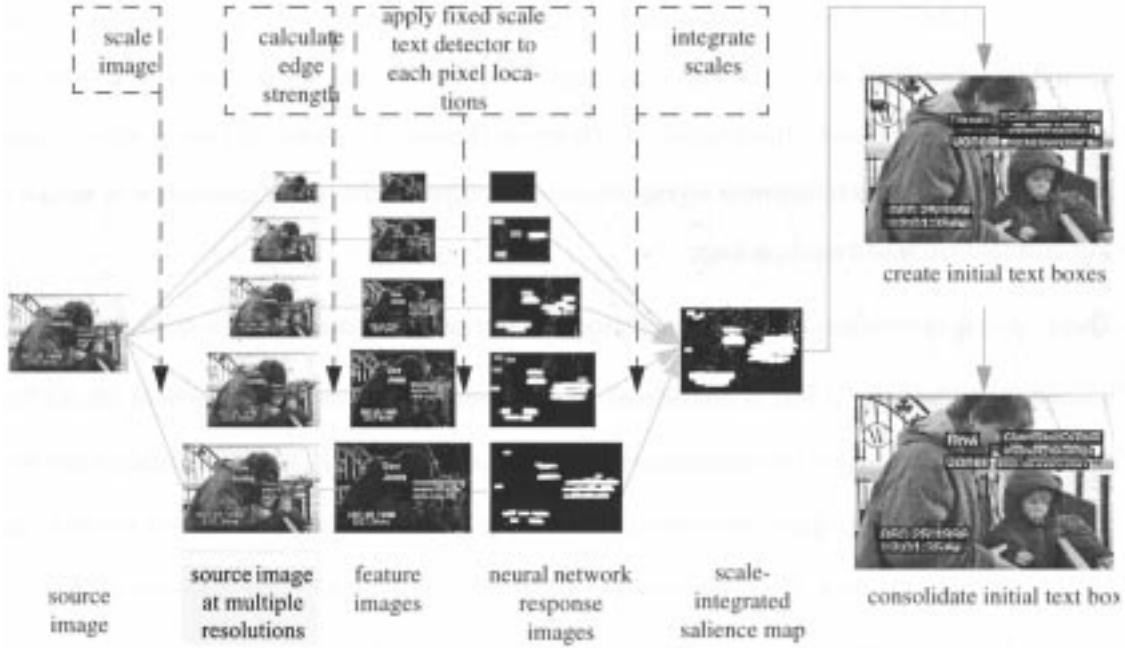
Fig. 1. Scale- and position-invariant text localization.
