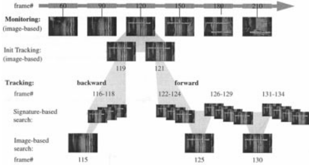
Fig. 6. Relationship between video monitoring (stage 1) and text tracking (stage 2).
