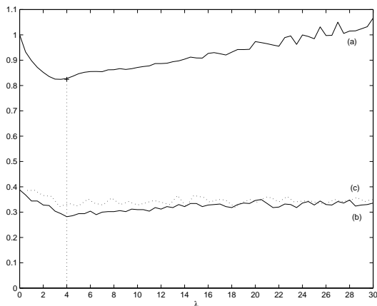
Figure 5: Threenorm. Cost \phi = \psi . \eta = 0.1 . n = 100 . m = 500 . Plot of (a) A^\lambda(\widehat{f}_n^\lambda) with MARGINBOOST. L_1 for various \lambda 's, (b) test error with MARGINBOOST. L_1 for various \lambda 's, (c) test error with one run of MARGINBOOST (unnormalized weights) where the test error is plotted as a function of the sum of the weights of the combined classifier denoted by \lambda_T .
