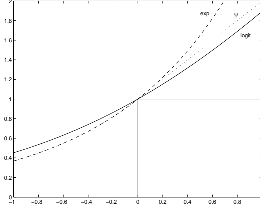
Figure 1: Bounding the step function with different cost functions \phi = \text{exp}, \psi, \text{logit} .
