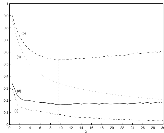
Figure 3: Threenorm. Cost \phi = \psi . n = 500 . m = 1000 . Plots of (a) A_n^\lambda(\widehat{f}_n^\lambda) . (b) A^\lambda(\widehat{f}_n^\lambda) . (c) training error. (d) test error.
