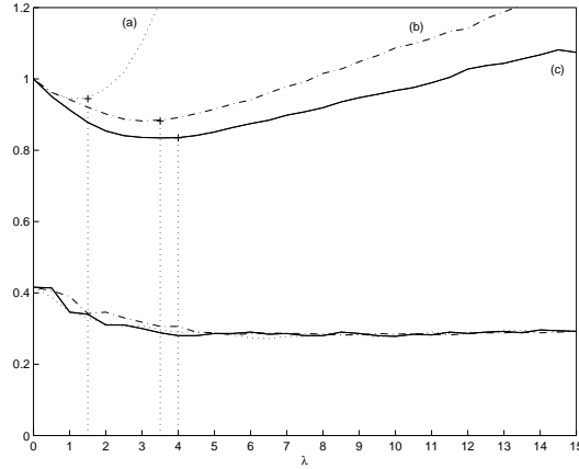
Figure 2: Threenorm. \eta = 0.1 . n = 100 . m = 500 . Plots of the cost A^\lambda(\widehat{f}_n^\lambda) (upper curves) and test error (lower curves) for various cost functions (a) exp, (b) logit, (c) \psi .
