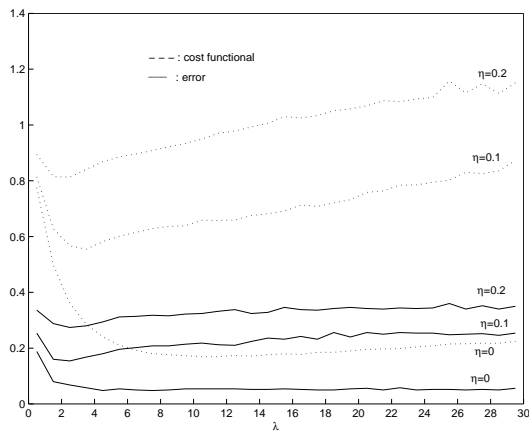
Figure 4: Twonorm. Cost \phi = \psi . n = 100 . m = 500 . Plots of A^\lambda(\hat{f}_n^\lambda) (dotted lines) and of the test error (solid lines) for levels of noise \eta = 0, 0.1, 0.2 .
