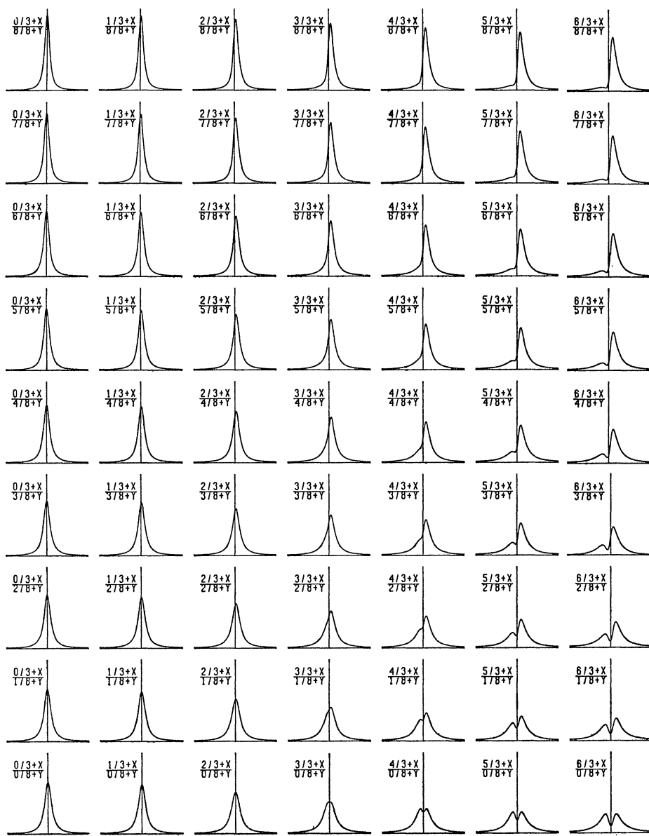
FIG. 1. Graphs of the density of (a+x)/(b+y) , where a > 0 , b > 0 and x, y are independent, standard normal random variables. The formula for the density is in equation (5). Values a = 0/3, 1/3, \dots, 6/3 and b = 0/8, 1/8, \dots, 8/8 were chosen so as to represent the possible shapes of the density function.
