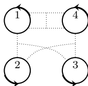
Figure 8: A diagram contributing to G_4^{(2)}
