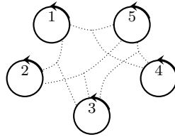
Figure 5: A diagram contributing to F_5^{(2)}
