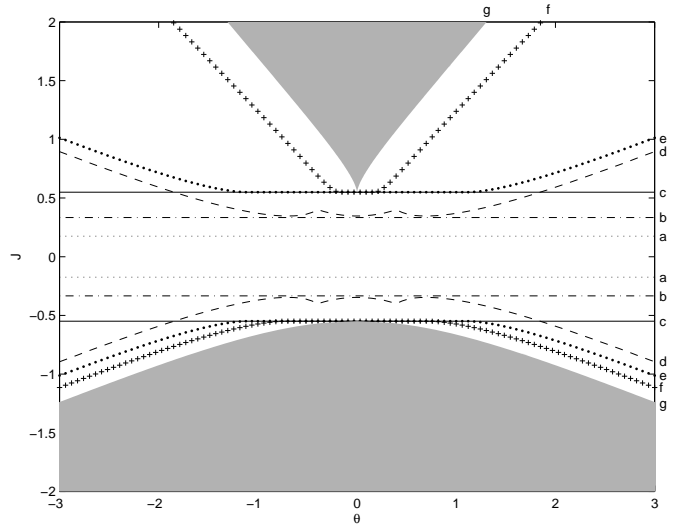
Fig. 4. Comparison of various LBP convergence bounds for the fully connected N = 4 binary Ising model with uniform coupling J and uniform local field \theta . (a) Heskes’ condition (b) Simon’s condition (c) spectral radius condition (d) Dobrushin’s condition (e) improved spectral radius condition for m = 1 (f) improved spectral radius condition for m = 5 (g) uniqueness of Gibbs’ measure condition. See the main text (section VI-A) for more explanation.
