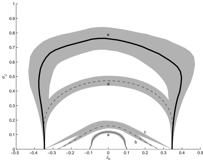
Fig. 5. Comparison of various bounds for LBP convergence for toroidal Ising model of size 10 \times 10 with normally distributed couplings J_{ij} \sim \mathcal{N}(J_0, \sigma_J) and zero local fields. (a) Heskes’ condition (b) Dobrushin’s condition (c) \ell_1 -norm condition (d) spectral radius condition (e) empirical convergence. See the main text (section VI-B) for more explanation.
