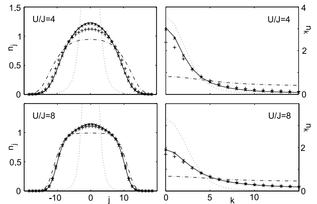
FIG. 2. Density and (quasi)-momentum distributions for interaction strengths U/J = 4 and 8 . Here, \beta J = 1 , L = 40 , N = 21 , and M = 10 . Numerical results were obtained for q = 2 (plus-signs), q = 3 (crosses), and q = 4 (solid line). For comparison, the distributions for U/J = 0 (dotted lines) and U/J \rightarrow \infty (dash-dotted lines) are also included.
