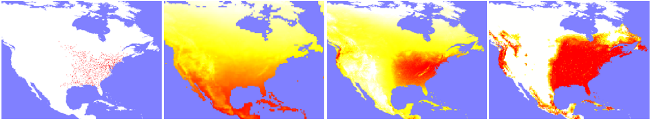
Figure 1. Left to right: Yellow-throated Vireo training localities from the first random partition, an example environmental variable (annual average temperature, higher values in red), maxent prediction using linear, quadratic and product features, and GARP prediction. Prediction strength is shown as white (weakest) to red (strongest); reds could be interpreted as suitable conditions for the species.
