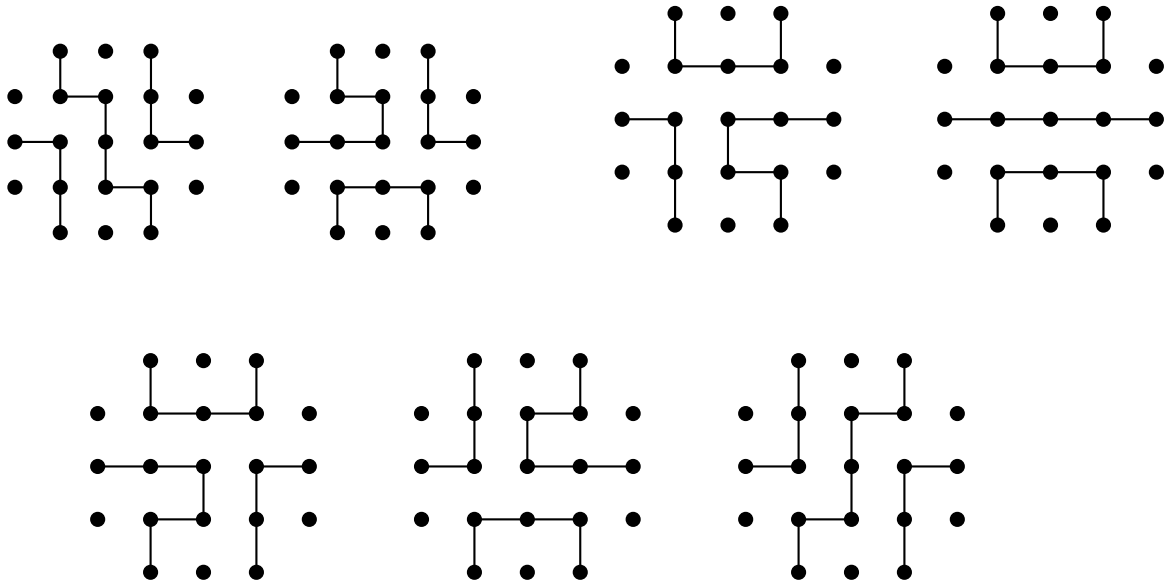
Figure 14: The seven FPL states of order 3.
