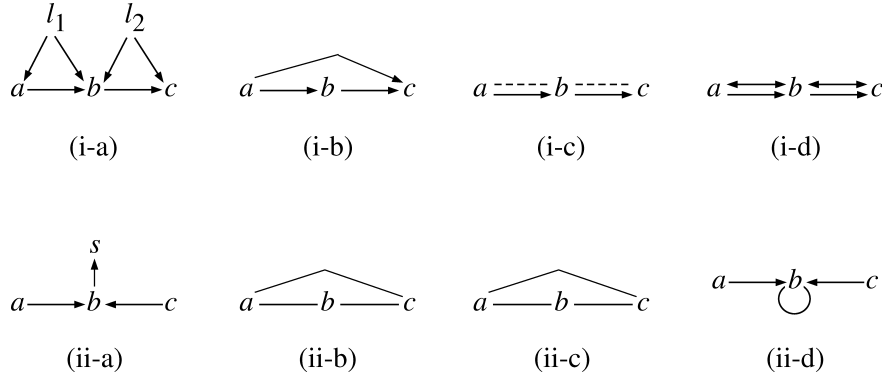
FIG. 18. (i-a) A DAG generating process \mathcal{D}_1 ; (i-b) the ancestral graph \mathcal{D}_1[\emptyset] ; the summary graph (i-c) and MC-graph (i-d) resulting from marginalizing l_1, l_2 in \mathcal{D}_1 . (ii-a) A DAG generating process \mathcal{D}_2 ; (ii-b) the ancestral graph \mathcal{D}_2[\emptyset] ; the summary graph (ii-c) and MC-graph (ii-d) resulting from conditioning on s in \mathcal{D}_2 .
