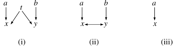
FIG. 10. (i) A simple DAG model, \mathcal{D} ; (ii) the graph \mathcal{D}_{[t]}^{\emptyset} ; (iii) the graph \mathcal{D}_{\emptyset}^{\{t\}} .
