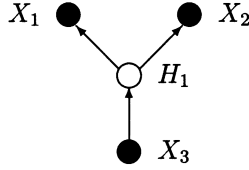
FIG. 8. A triadic nest with one hidden variable.
