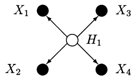
FIG. 5. A directed tree with one hidden variable.
