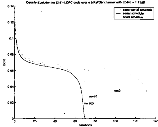
Fig. 2: Density Evolution analysis over Gaussian channel
