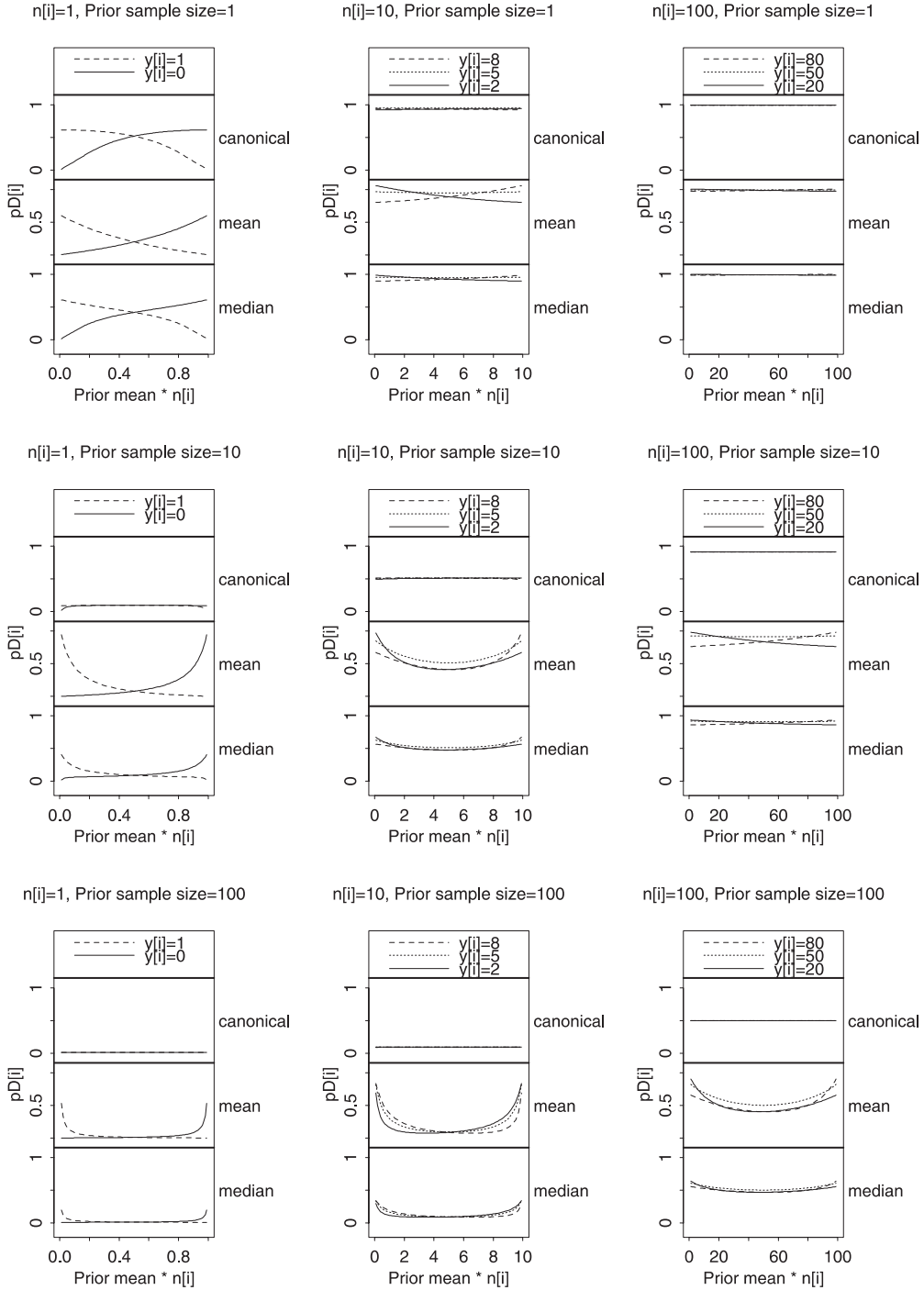
Fig. 1. Binomial likelihood—contribution of the i th group to the effective number of parameters under various parameterizations (canonical p_{D_i}^c , mean p_{D_i}^\mu and median p_{D_i}^{\text{med}} ) as a function of the data (sample size n_i and observed proportion y_i/n_i ) and prior (effective prior sample size a+b and prior mean a/(a+b) ): we are seeking agreement between alternative parameterizations with little dependence on data
