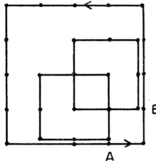
FIG. 8. "Forbidden" domain giving a finite contribution to g(x) .
